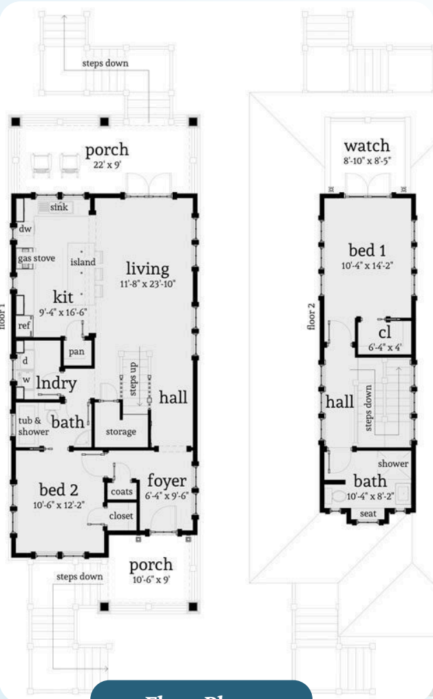
Floor Plans
